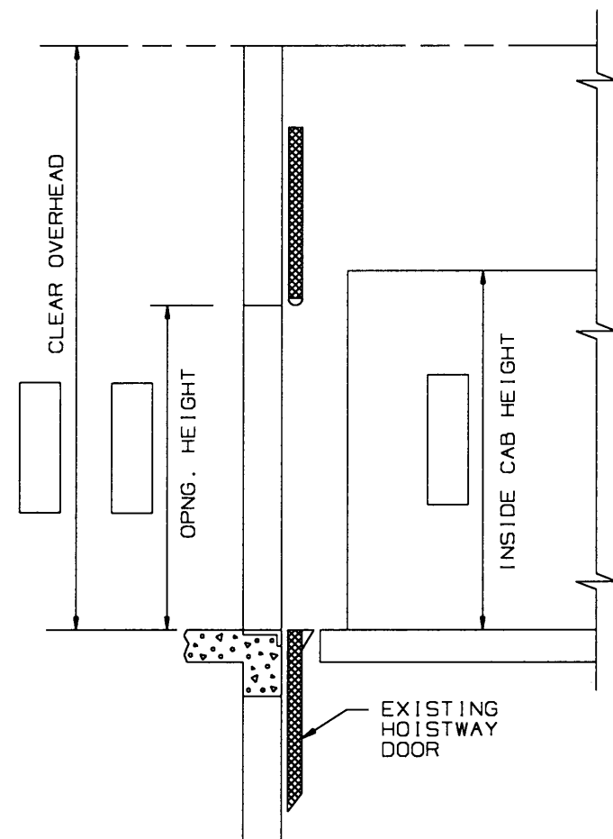
SECTION THRU HOISTWAY
