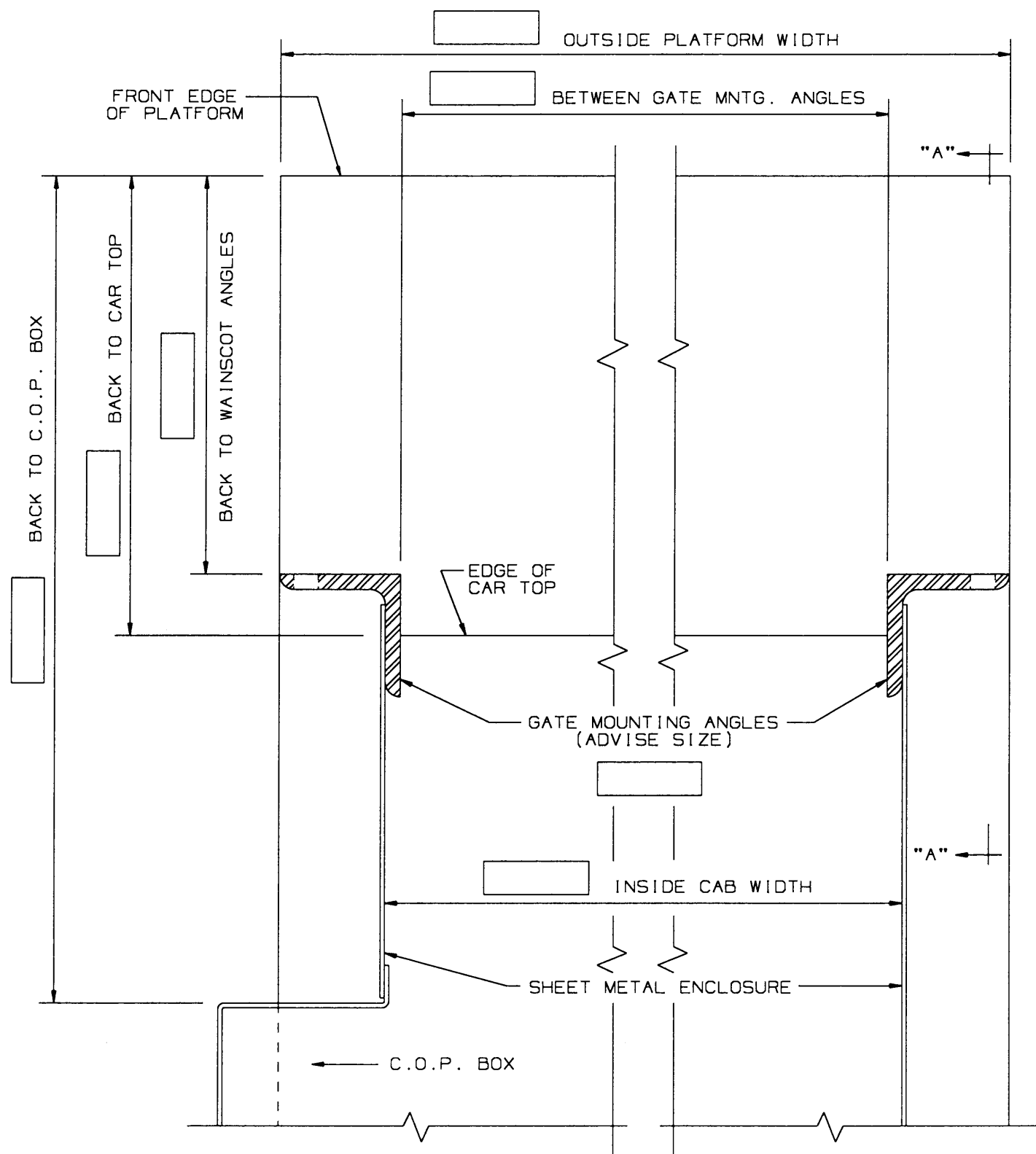
PLAN OF CAR ENCLOSURE
